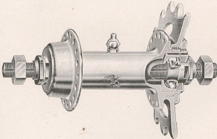
Modell No. 21 - Hinterrad-Nabe DCN
