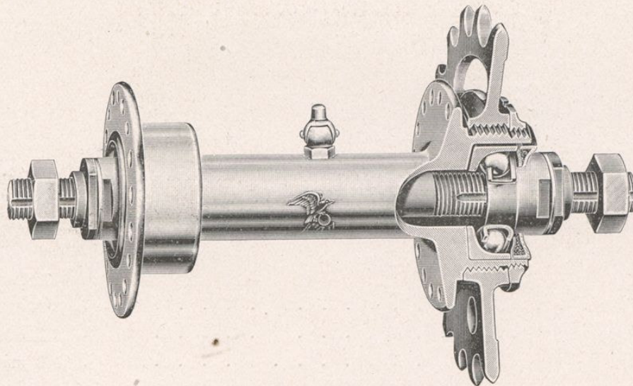
Modell No. 81 - Hinterrad-Nabe
