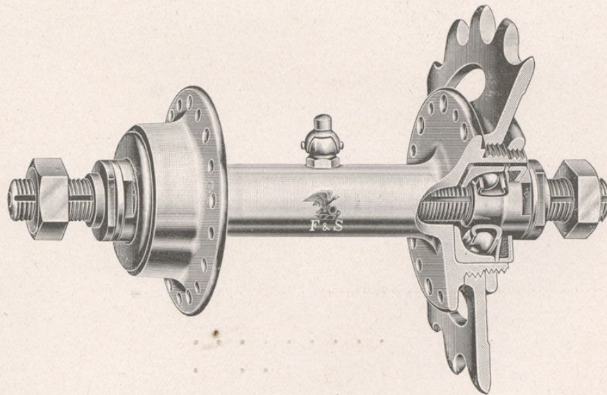
Modell No. 41 - Hinterrad-Nabe H
